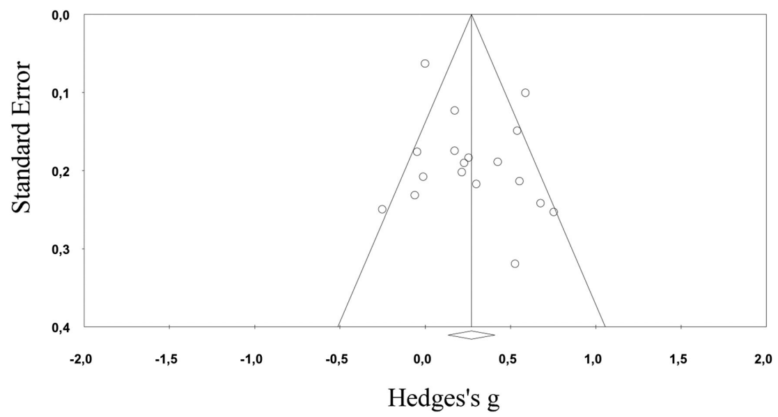
Figure A1. Funnel plot of Standard Error by Hedges's g .
